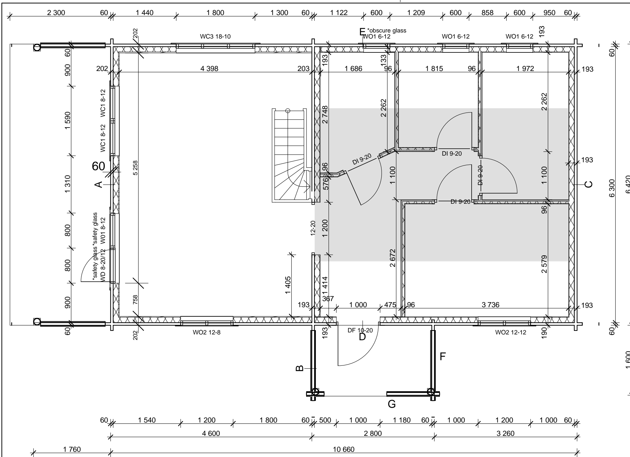
Measurements plan
